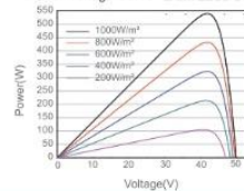
Power-Voltage Curve JAM72S30-540/MR/1500V
