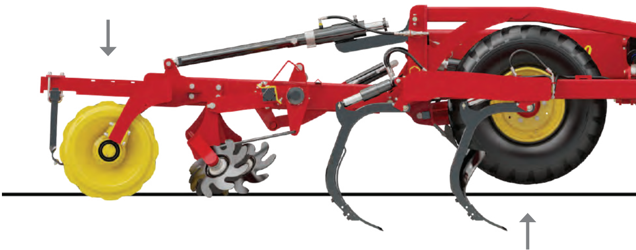
Full-depth – all weight on packer
